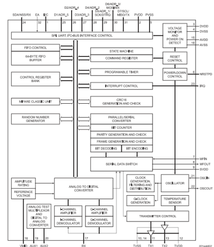
Gambar 5. Detail Diagram Blok MRFC522
