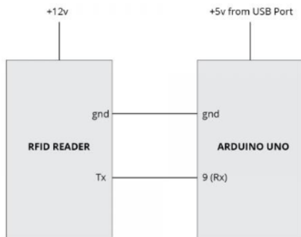
Gambar 7. Interfacing RFID Reader to Arduino
