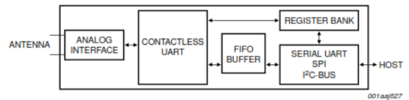
Gambar 4. Diagram Block MRFC522
