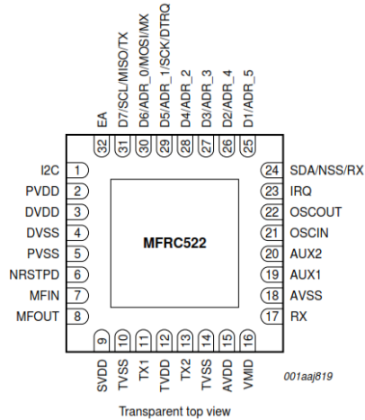
Gambar 6. Pinning configuration
