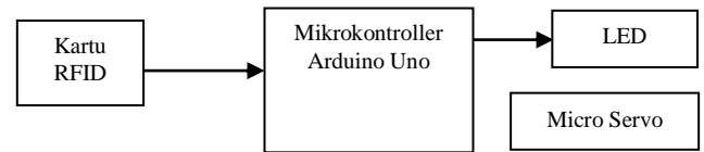
Gambar 2. Diagram Blok sistem auto lockdoor berbasis Arduino Uno
